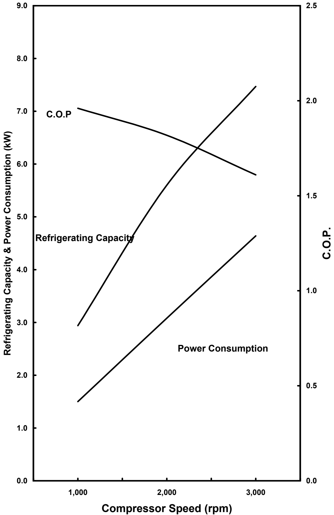
SD7H15 Performance
